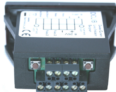
Rear view of the DCLIB
